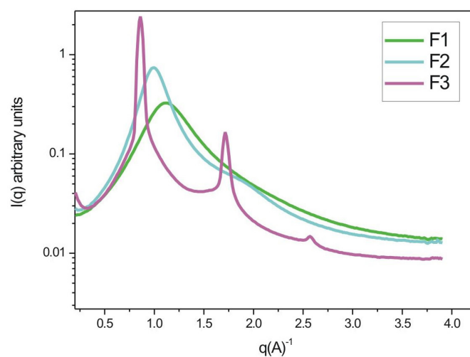
FIGURE 8 – SAXS profiles of systems stabilized by 80, 70 and 60% (PPG-5-Ceteth-20); 10, 20 and 30% (water) and 10% (oleic acid).
