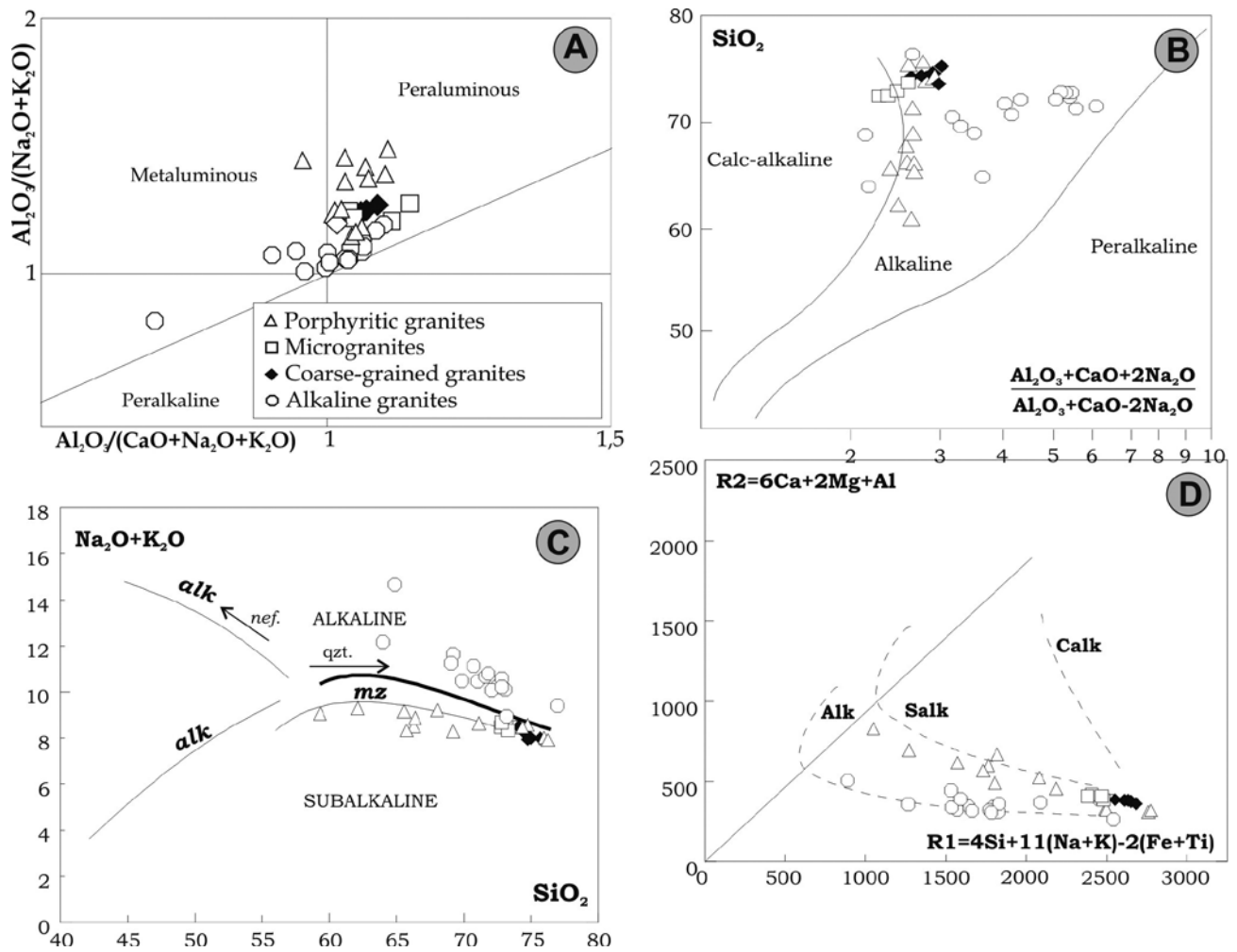
Figure 7. A. Alumina saturation (Shand) index with fields suggested by Maniar and Piccoli (1989). B. Alkalinity vs. SiO_2 after Wright (1969), showing the transitional character of some of the porphyritic granites. C. TAS diagram. See text for discussion of divisions and trends. D. R_1 - R_2 diagram according to La Roche et al. (1980).
