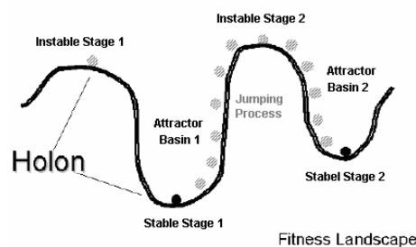
Figure 2 - Illustration of a “Fitness Landscape” and the attractor basins. Adapted from Eijnatten (2003).
