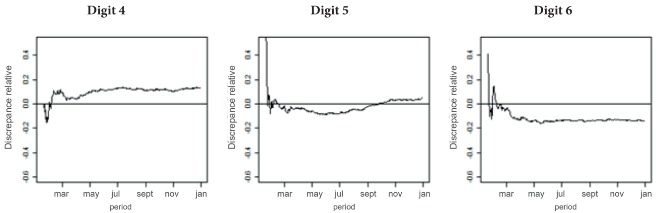
Figure 8 Time series graphs of relative discrepancies for state S2 in the period from 01/17/2010 to 12/31/2010 for digits 4, 5, and 6.
