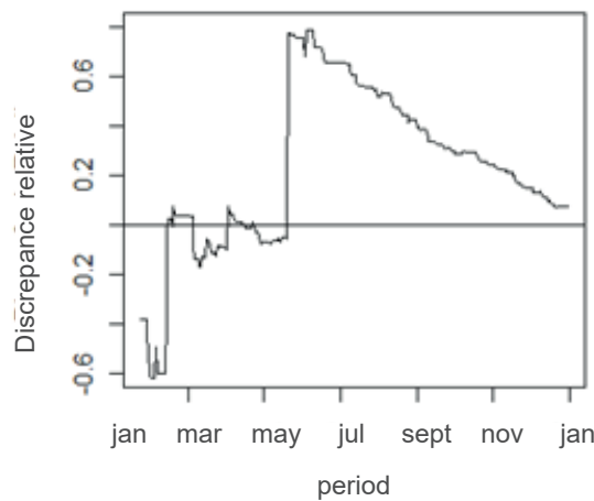
Figure 15 Graph of relative discrepancies observed for the digit 7 in the first significant position, considering MU 8 from state S2 in the period from 01/31/2010 to 12/31/2010.
