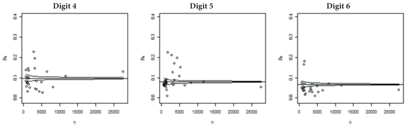
Figure 2 Graphs of observed frequencies for state S1 at the end of 2010 for the digits 4, 5, and 6. Source: Prepared by the authors.
