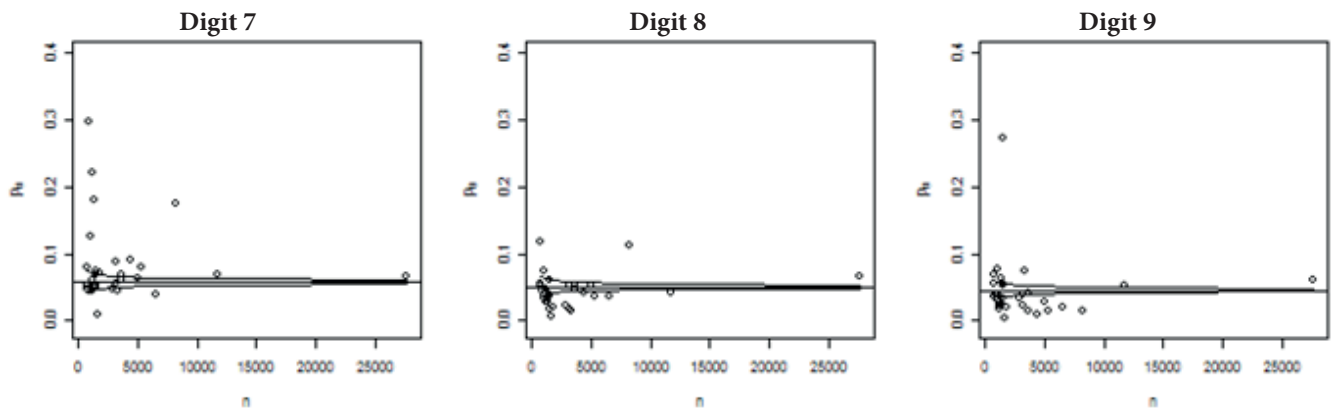
Figure 3 Graphs of observed frequencies for state S1 at the end of 2010 for the digits 7, 8, and 9. Source: Prepared by the authors.
