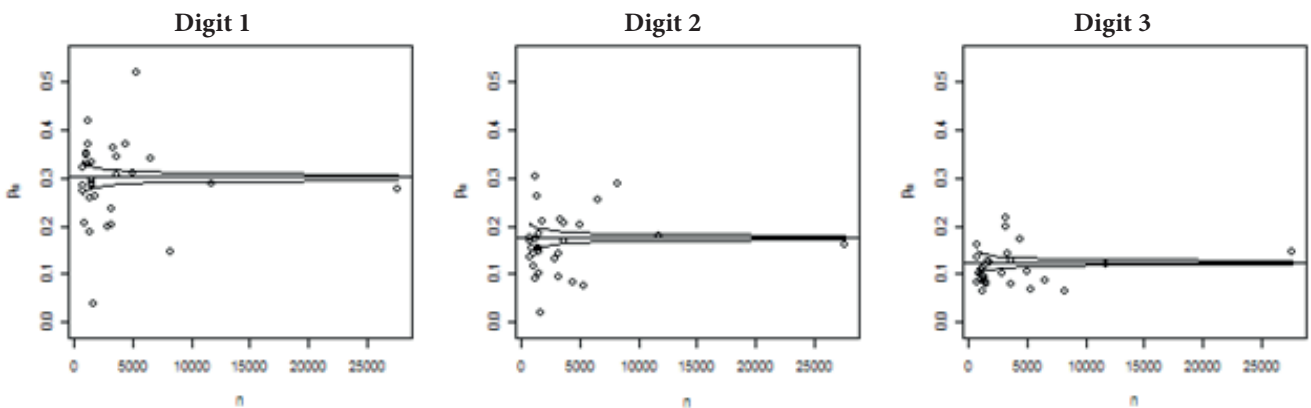
Figure 4 Graphs of observed frequencies for state S2 at the end of 2010 for the digits 1, 2, and 3. Source: Prepared by the authors.
