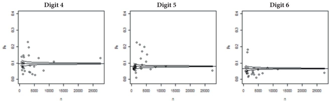
Figure 5 Graphs of observed frequencies for state S2 at the end of 2010 for the digits 4, 5, and 6. Source: Prepared by the authors.
